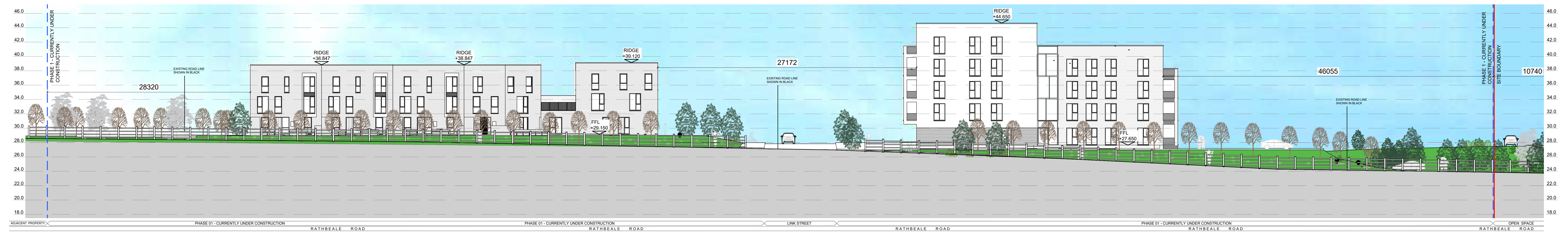
PROPOSED SITE SECTION/CONTIGUOUS ELEVATION A-A (PART A) 1:200 @ A0
